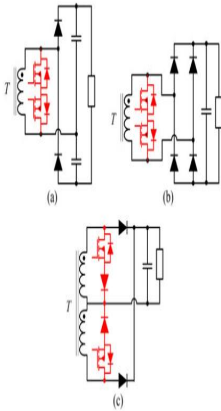
Fig. 5. Derived ABR topologies: (a) voltage-doubler, (b) full-bridge, and (c) center-tapped.
