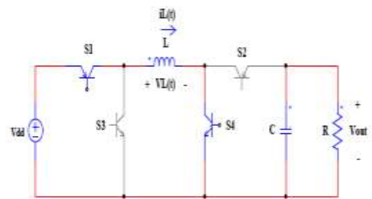
Fig.3 (a) Charging interval of buck mode. (b) Discharging interval of buck mode.
