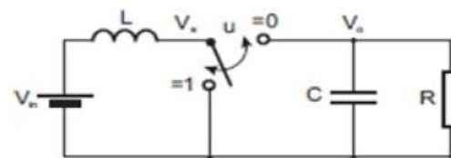
(b) Boost
