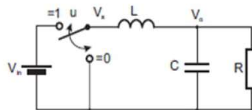
(a) Buck
