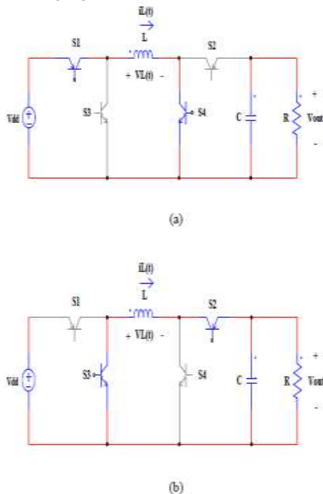
Fig.4 (a) Charging interval of boost mode. (b) Discharging interval of boost mode
