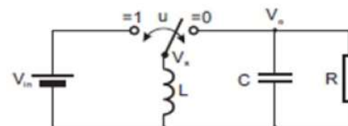
(c) Buck-boost
