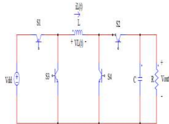
Fig.2 Proposed converter circuit.
