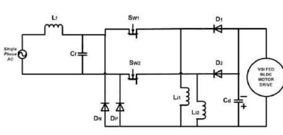
Fig 1 : Proposed Converter
